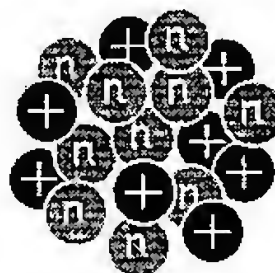
^{18}\text{O} NUCLEUS
