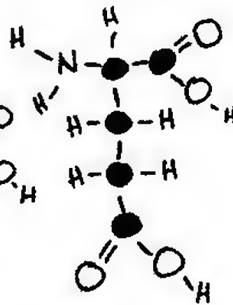
GLUTAMIC ACID
