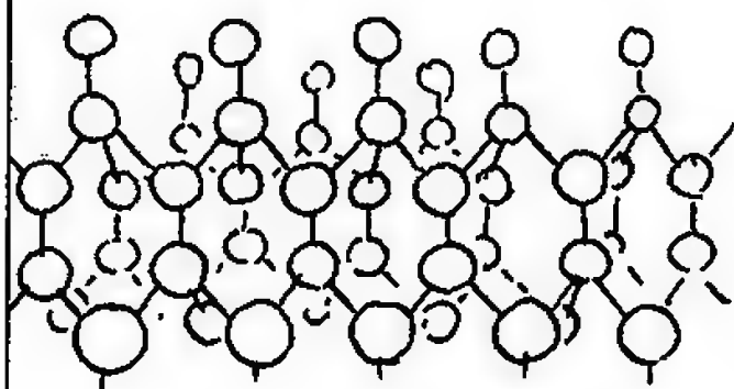
DIAMOND
